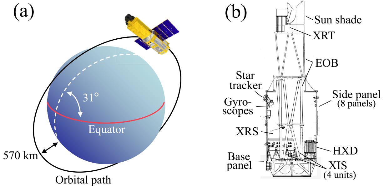
Fig. 5.1.—: (a) Schematic view of the Suzaku satellite in orbit (Mitsuda et al. 2007). (b) Schematic cross-section of Suzaku with the internal structure after the EOB extension (Mitsuda et al. 2007).
