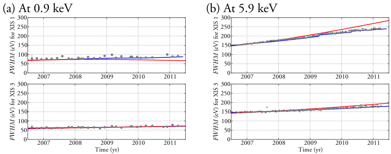
Fig. 5.15. —: Long-term trend of energy resolution at (a) 0.9 keV and (b) 5.9 keV. Upper and lower panels show FWHM for XIS 1 and XIS 3, respectively. The observed data are shown with gray dots while the best-fit models with the original calibration by Uchiyama et al. (2009) and with the improved calibration method are shown with red and blue curves, respectively.
