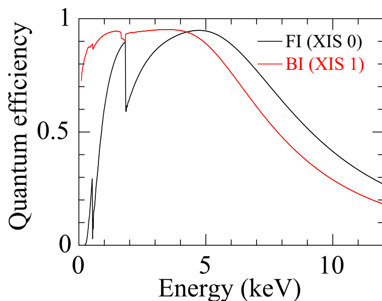
Fig. 5.10. —: Quantum efficiencies of the XIS as a function of incident photon energy. The black and red curves are for XIS 0 (FI) and XIS 1 (BI) respectively (Koyama et al. 2007a). The effect of contaminant on the OBF is not included.
