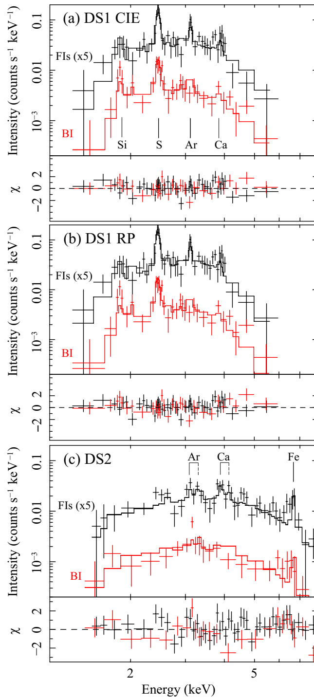
Fig. 6.3. —: Background-subtracted XIS spectra (pluses) and the best-fit models (histograms) of (a) DS1 with the CIE plasma model, (b) DS1 with the recombining plasma model, and (c) DS2 with the CIE plasma model. XIS merged FI and BI spectra are shown in black and red, respectively. Black spectra are scaled upward by a factor of 5 for clarity.
