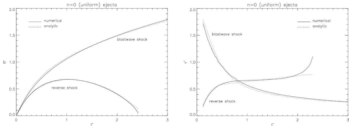
Fig. 3.3. —: Shock positions (left) and velocities (right) for blast wave and reverse shock in remnants of uniform ejecta (Truelove & McKee 1999). Note that the reverse shock velocity is measured in the frame of the unshocked ejecta ahead of it.
