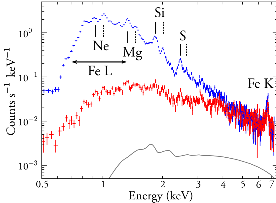
Fig. 8.3. —: Comparison of the source (blue) and the normalized background (red) spectra. For visibility, only merged spectra of FI (XIS 0 and XIS 3) are displayed. The solid and dashed black lines show the center energies of K\alpha lines from He-like and H-like ions, respectively. The gray line indicates the CXB spectrum.
