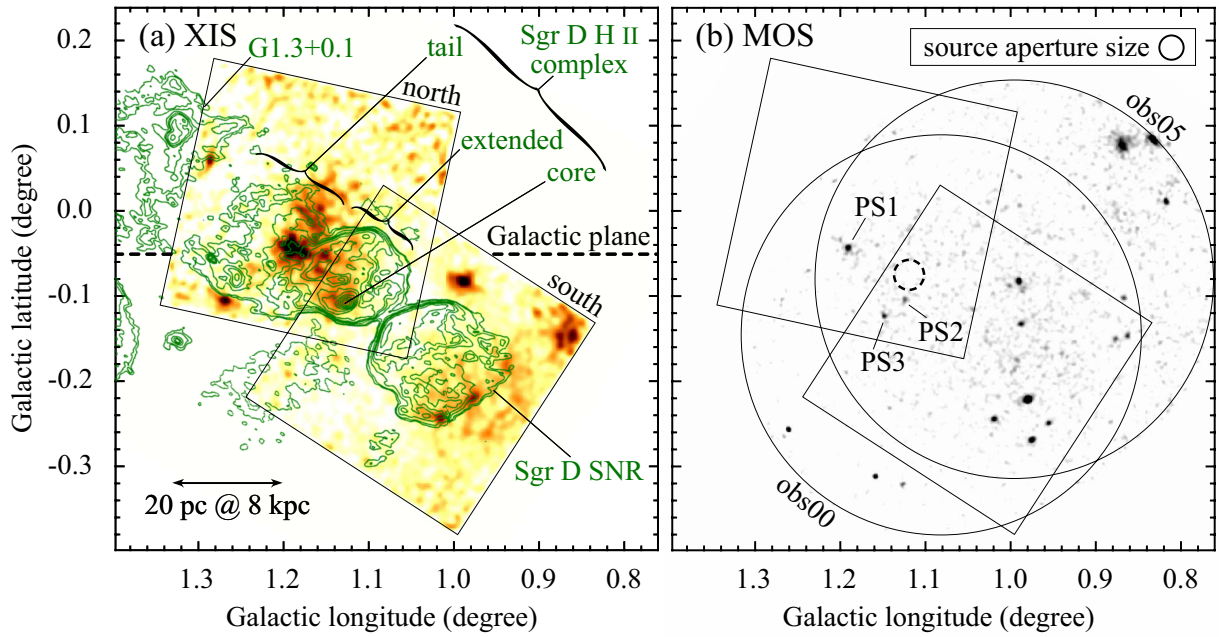
Fig. 6.1. —: Wide-band (0.7–5.5 keV) smoothed images by the (a) XIS and (b) MOS shown with the logarithmic intensity scale. Overlaid green contours in (a) are an 18 cm radio continuum map from the Very Large Array (VLA; Mehringer et al. 1998). The point source extraction aperture and background accumulation region are respectively shown with solid and dashed circles in the panel (b). For the XIS image, we merged events with the three CCDs, subtracted the NXB (Tawa et al. 2008), corrected for the vignetting, and mosaicked the two fields with different exposure times normalized. The FOVs are shown with two solid squares with 18' in length. For the MOS image, we merged two CCDs and mosaicked the two fields with normalized exposures. The fields are shown with two circles with 30' in diameter.
