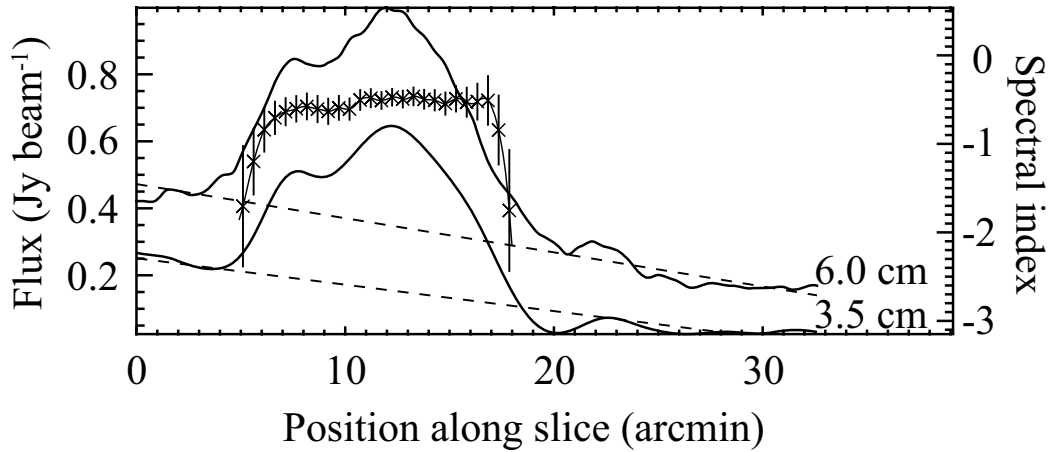
Fig. 6.4. —: Profiles of 3.5 cm and 6.0 cm intensity (solid curves) and the spectral index (crosses) between the two bands along the slice shown in figure 6.6a. Background (dashed lines) is derived by linearly fitting the slope at the two sides of the source region, where the indices are computed. The error bars indicate 1\sigma uncertainty.
