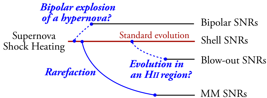
Fig. 10.1. —: Schematic view of the missing branches in the SNR evolution.
