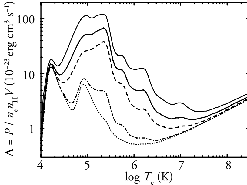
Fig. 3.1. —: Cooling coefficient for an optically thin thermal plasma (Sutherland & Dopita 1993). Curves with 1, 0.3, 0.1, 0.01, and 0.001 times solar abundances are shown from top to bottom as a function of plasma temperature.
