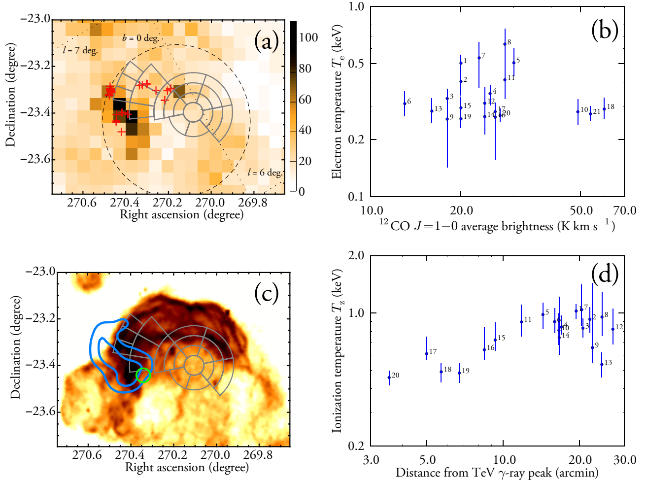
Fig. 9.2. —: The spatial correlations between RP and other structures. (a) The distribution of the interacting molecular clouds. The colormap shows the CO J=1-0 molecular line intensity by NANTEN with linear scale in units of \text{K km s}^{-1} , integrated over 0-10 \text{ km s}^{-1} . The CO map is taken from figure 2 of Aharonian et al. (2008). The red crosses are the positions of the OH (1720 MHz) masers (Claussen et al. 1999). The black dashed circle indicate the rough boundary of the radio shell. (b) A comparison between CO J=1-0 average brightness and T_e . (c) The distribution of the GeV and TeV \gamma -ray emission overlaid on the radio 90-cm continuum image in the same scale with figure 8.5b. The blue contours are the TeV \gamma -ray significance map by H.E.S.S. at 4- and 5- \sigma levels (Aharonian et al. 2008), while the green circle is the 1- \sigma error region of the GeV \gamma -ray peak by Fermi (Abdo et al. 2010b). (d) A comparison between the projected distances from TeV \gamma -ray peak at the northeast of the remnant and T_z . The labels in (b) and (d) indicate the sector numbers (see figure 8.5b).
