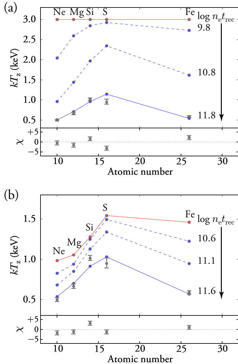
Fig. 9.3.— Time evolution of T_z in RPs with the initial conditions of (a) T_{z0} = 3.0 keV for all elements and (b) T_{z0} realized by an IP with T'_c = 10 keV and n_e t_{\text{ioni}} = 10^{11} s \text{cm}^{-3} . The gray circles with bars show the observed T_z with the 1\text{-}\sigma statistical errors. The direction of evolution as a function of n_e t_{\text{rec}} is indicated by the vertical arrows. The solid lines in red and blue respectively show the initial and final states while the dashed blue lines show transitional states.
