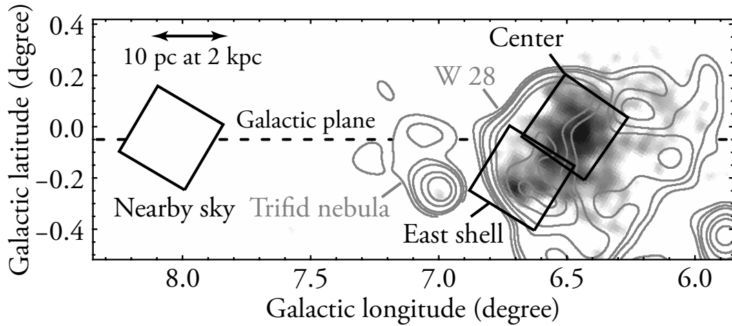
Fig. 8.1. —: Wide-field X-ray image retrieved from the ROSAT All Sky Survey in grayscale (Snowden et al. 1995). Overlaid contours are the radio continuum map at 1.4 GHz by the Very Large Array (Dubner et al. 2000). The XIS FOVs are shown with the solid squares.
