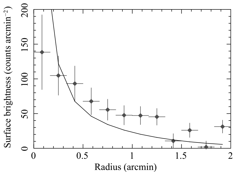
Fig. 6.5.— Radial profile of the background-subtracted intensity around PS2 (solid pluses with dots), which is fitted with a simulated radial profile of a point-like source at the same detector position (solid curve). The energy range of 2.0–5.5 keV is used to suppress the emission by PS3. The observed profile is constructed from the north field data.
