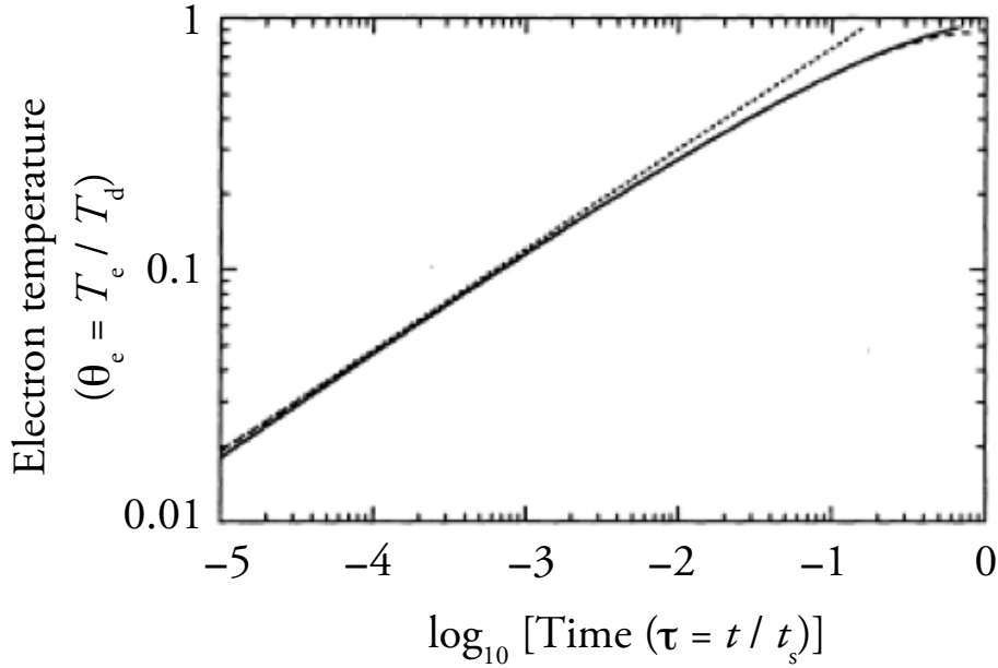
Fig. 4.2.— Evolution of the normalized electron temperature \theta_e due to Coulomb collisions with the ions in the post-shock region (Masai 1994). The solid, dashed, and dotted lines indicate the analytic solution (equation 4.57) and its approximations up to the second (equation 4.60) and the first order (equation 4.61), respectively.
