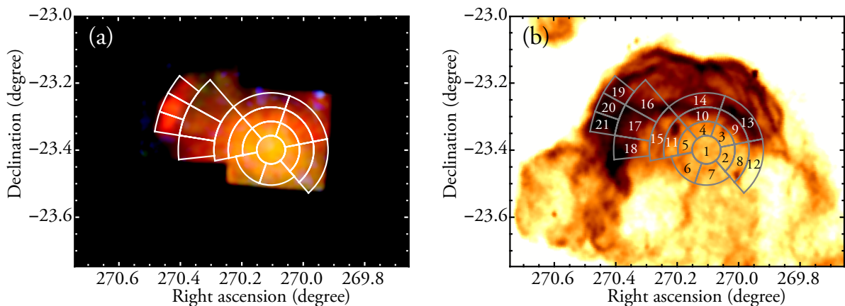
Fig. 8.5.— The divided sectors for the spatially resolved spectral analysis (white regions) overlaid on (a) the X-ray images and (b) the radio 90-cm continuum image (Brogan et al. 2006) of W28. The red, green, and blue colors in (a) show the soft (0.5–2.0 keV), medium (2.0–5.0 keV), and hard (5.0–8.0 keV) X-rays, respectively. The labels in the panel (b) indicate the sector numbers.
