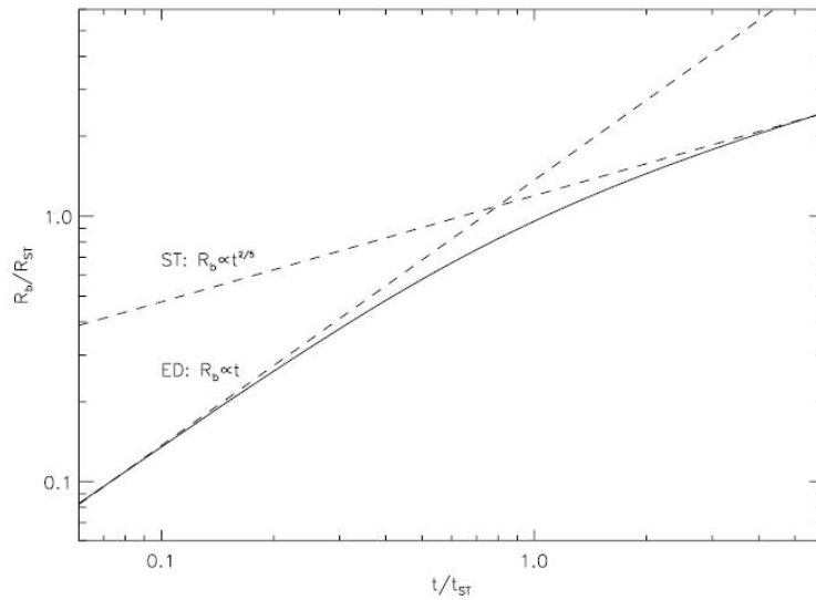
Fig. 3.2. — Time evolution of shock wave position (solid curve) derived by a simulation of uniform ejecta expanding into a uniform ISM (Truelove & McKee 1999). The time and position are respectively normalized by the values at the transition ( t_{\text{ST}} and R_{\text{ST}} ) from ejecta-dominated (ED) free expansion phase to Sedov-Taylor (ST) phase. The time evolution in each phase is also given in dashed curves.
