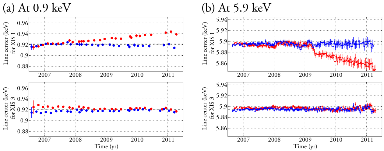
Fig. 5.14. —: Long-term trend of energy scale at (a) 0.9 keV and (b) 5.9 keV after the CTI correction. Upper and lower panels show the line center energies for XIS 1 and XIS 3, respectively. The data with different correction methods are shown: the results of the original method (Uchiyama et al. 2009) in red error bars and those of the upgraded CTI correction in blue error bars. The reference energy is also shown with dashed gray lines.
