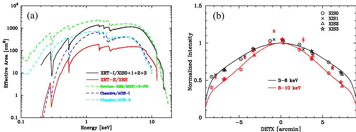
Fig. 5.5.— (a) Total effective area of the XRT combined with the XIS (Serlemitsos et al. 2007). Those of other X-ray missions are also shown for comparison. (b) Off-axis angle dependence of the effective area normalized at the optical axes in the soft and hard bands shown with black and red points, respectively (Serlemitsos et al. 2007). Data are obtained with the observations of Crab nebula. The solid lines show the simulated model.
