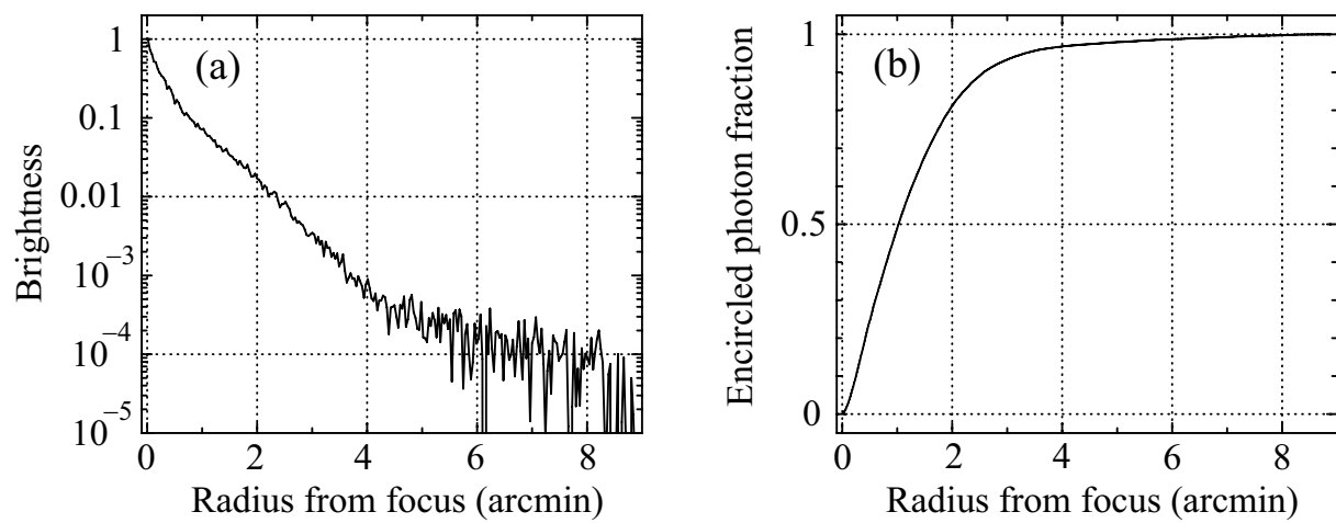
Fig. 5.7. —: Point spread function (PSF, left panel) and the encircled energy fraction (EEF, right panel) of the XRT (for XIS2) at the focal plane (Serlemitsos et al. 2007).
