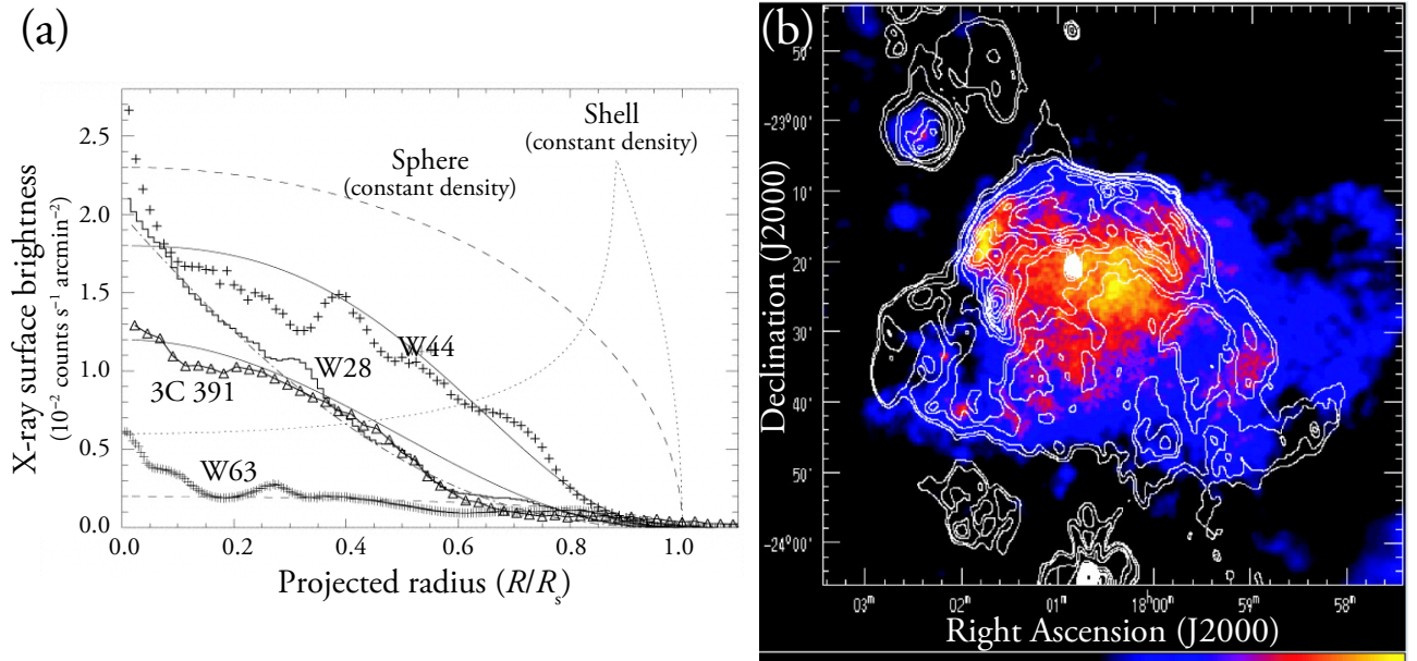
Fig. 2.2. — Structure of MM SNRs. (a) X-ray surface brightness profiles of the MM SNRs W 44, 3C 391, W 28, and W 63 with ROSAT. Model profiles for various density distributions are also plotted: a Sedov shell, a sphere with a constant density, and the best distributions for each remnant. The plot was made by Rho & Petre (1998). (b) A composite image of the MM SNR W 28 (Rho & Borkowski 2002). The X-ray and radio emission is shown in color and white contours, respectively.
