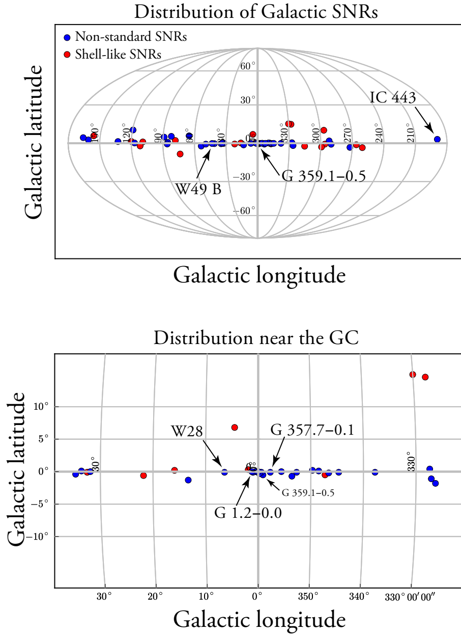
Fig. 2.3. —: Distribution of Galactic SNRs. 43 non-standard SNRs and 21 shell-like SNRs are plotted. Their positions are taken from Green (2009) and references therein. The recent results by the Suzaku GC mapping ( |l| < 2^\circ ) are also taken into account to compensate the information (SNRs in Sgr C: Tsuru et al. 2009, Sgr A: Mori et al. 2008, Sgr B1: Nobukawa et al. 2008, Sgr B2: Koyama et al. 2007b, Sgr D: Sawada et al. 2009). The location of the three known SNRs which exhibit recombining plasmas and our three targets are shown with arrows.
