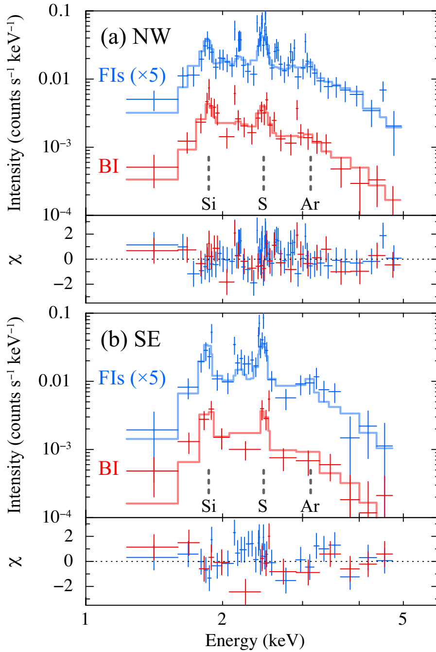
Fig. 7.3. —: (a) The background-subtracted spectra for NW. The FI and BI spectra are separately given by blue and red crosses, respectively. For visibility, the FI spectrum is multiplied by 5. The blue and red histograms are the best-fit model of FI and BI spectra, respectively. (b) Same as panel (a) but for SE.
