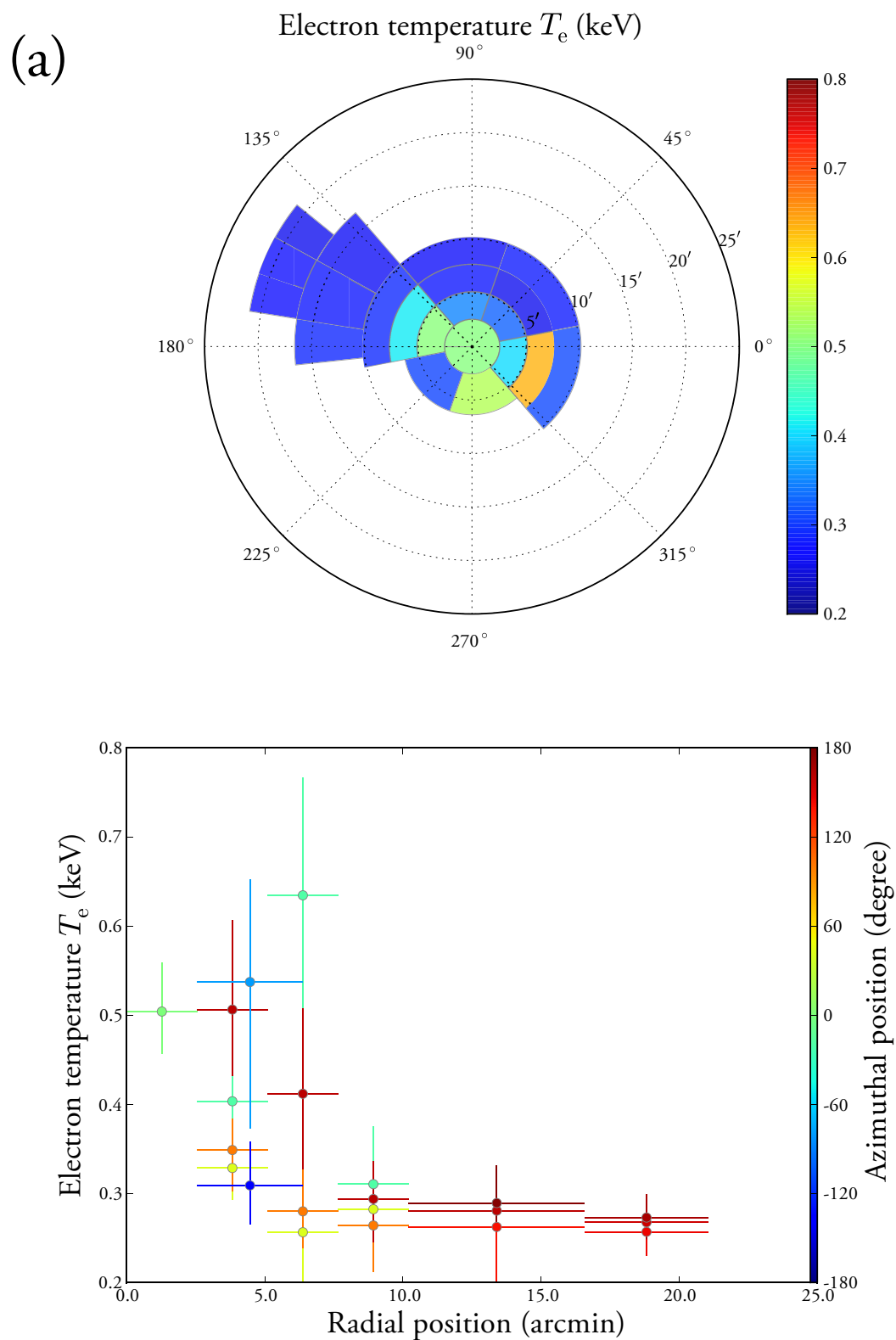
Fig. 9.1. —: The spatial variation of (a) the electron temperature and (b) the ionization temperature in W 28. Colormap in upper panels show the best-fit values while crosses in lower panels show the best-fit values and the statistical uncertainties with respect to the radial positions. The color of the crosses indicate the azimuthal positions.
